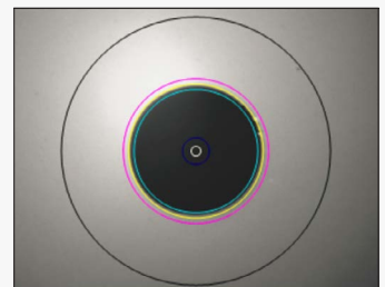
Step 3: Reinspect and mate the connectors Pristine end-faces compliant to IEC 61300-3-35 as seen through the FiberCheck™ Probe Microscope
