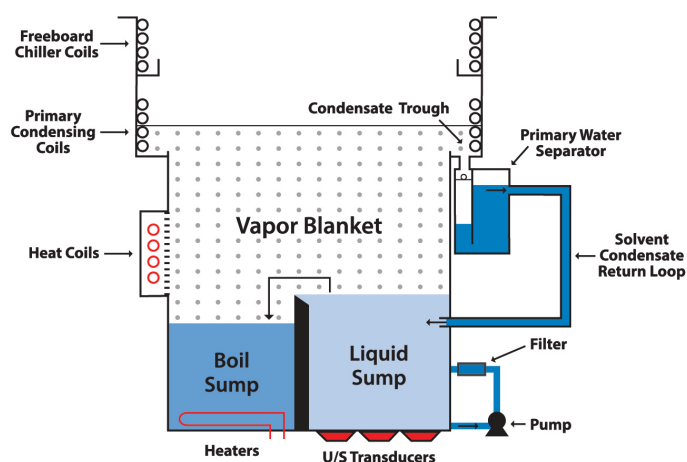
2-Sump Vapor Degreaser
